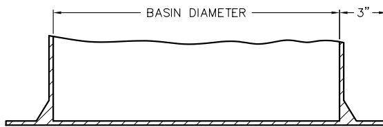
BOTTOM ANTI-FLOATATION FLANGE
