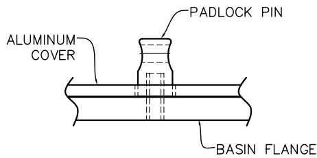
DETAILED SIDE VIEW OF PADLOCK PIN INSTALLED
