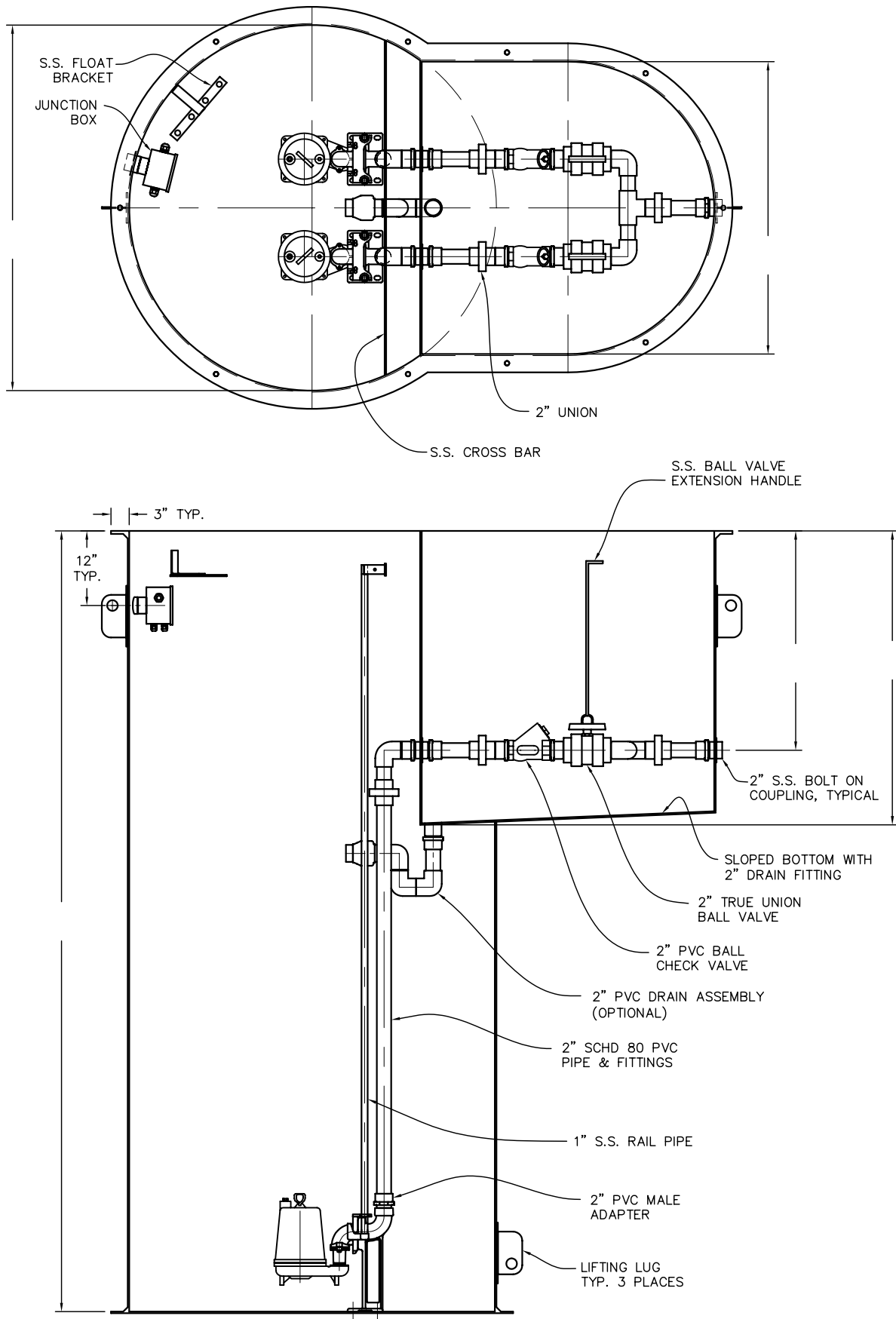
FOR 1 1/4", 1 1/2", OR 2" VERTICAL DISCHARGE PUMPS
