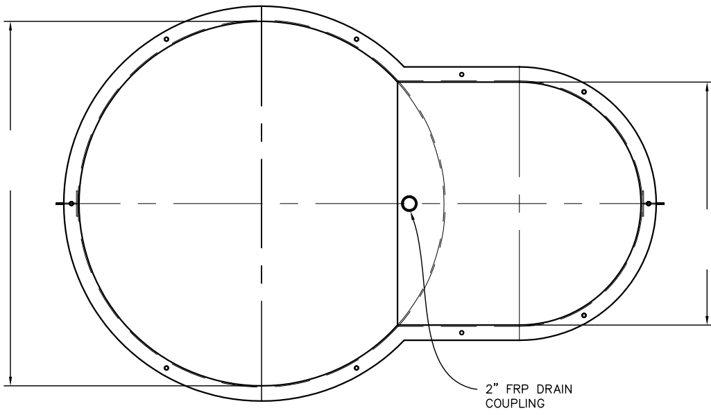
TOP VIEW
