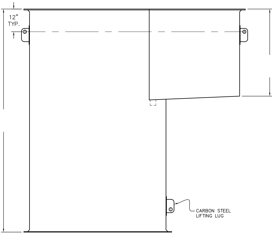
SIDE VIEW
