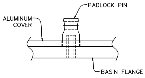
DETAILED SIDE VIEW OF PADLOCK PIN INSTALLED
