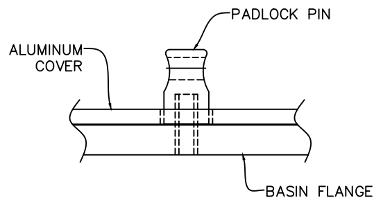
DETAILED SIDE VIEW OF PADLOCK PIN INSTALLED
