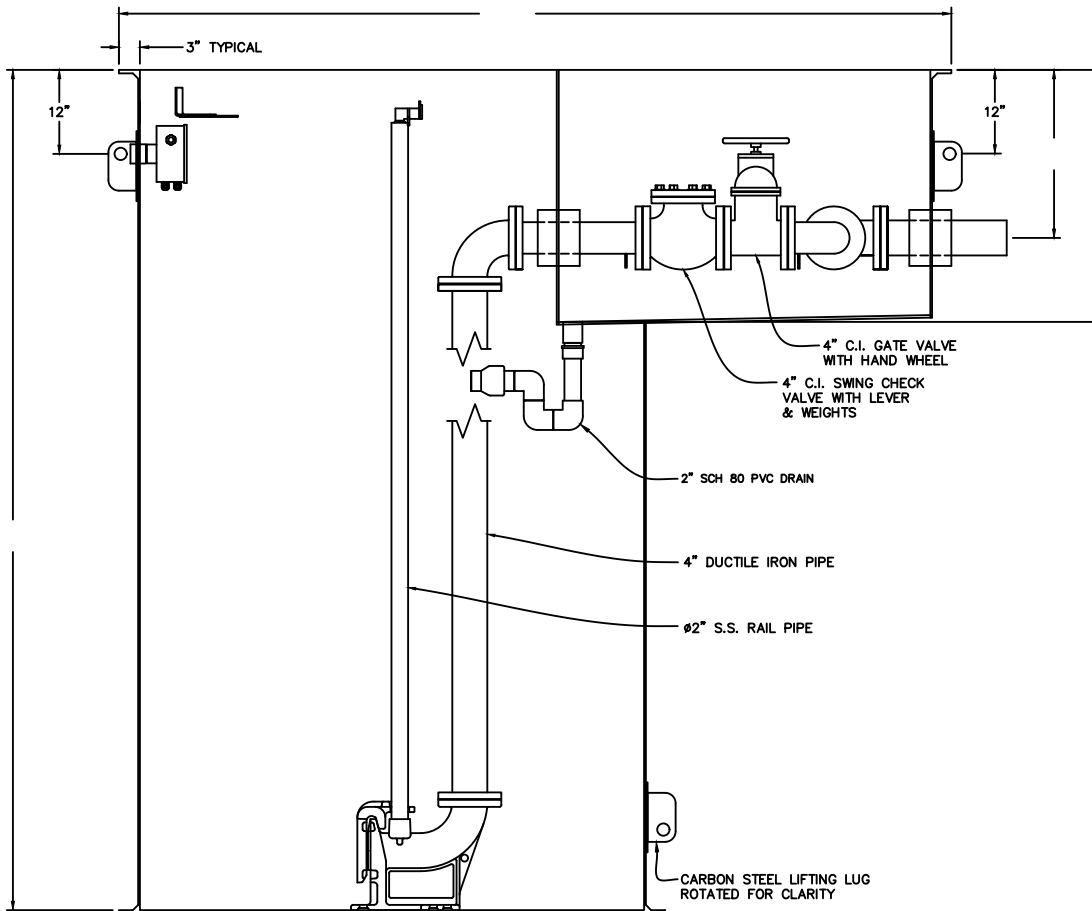
SECTIONAL ELEVATION VIEW
