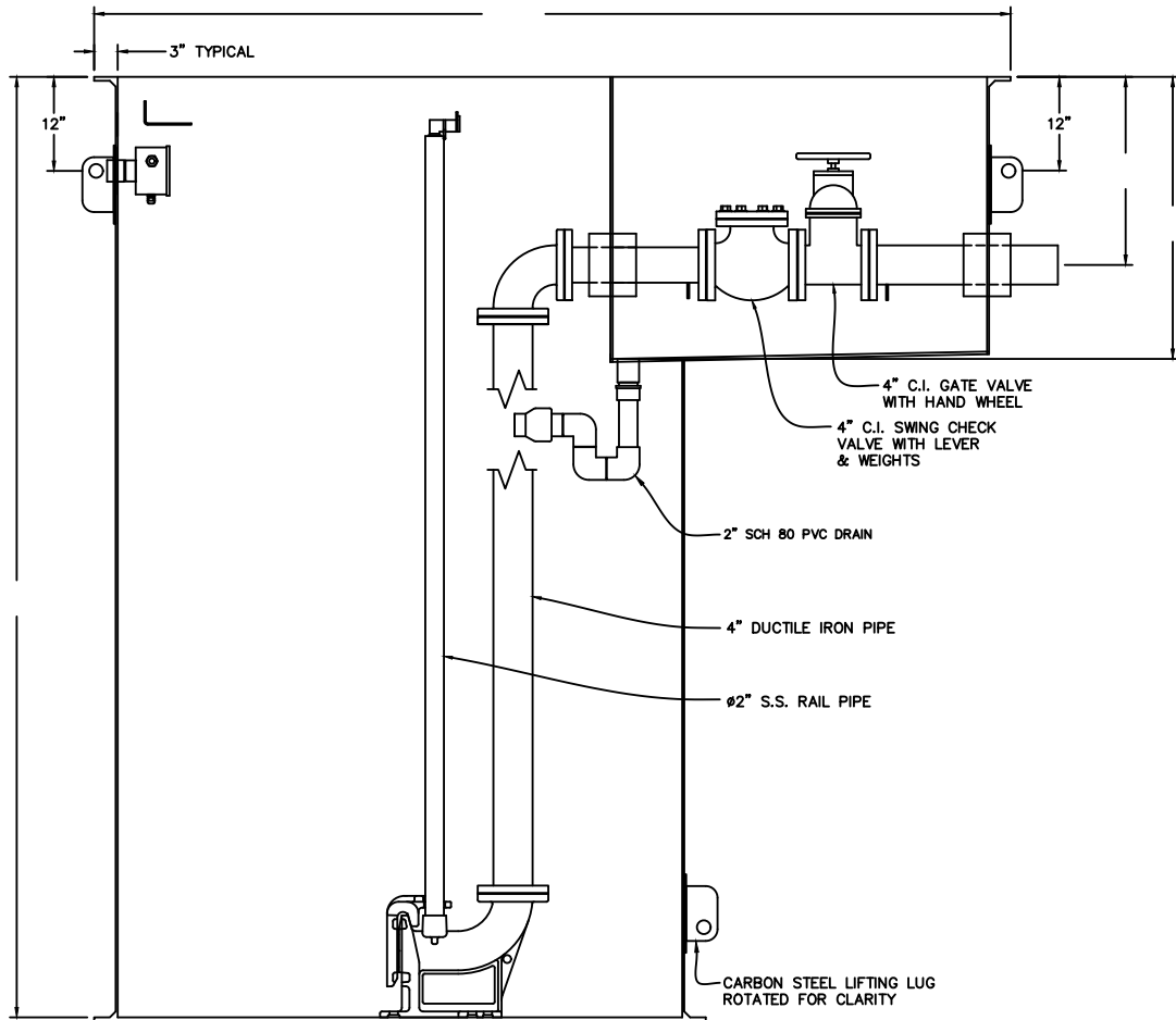
SECTIONAL ELEVATION VIEW
