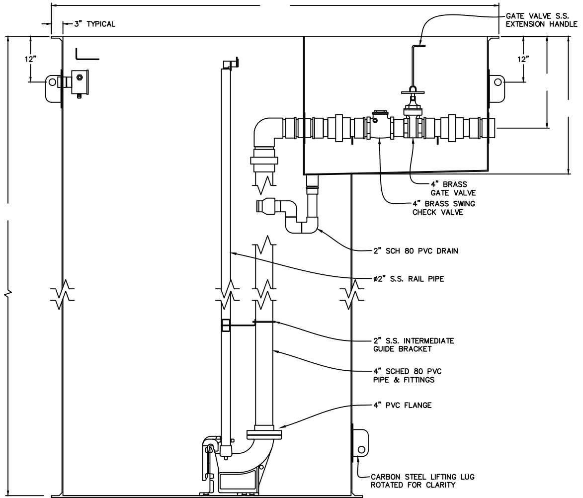
SECTIONAL ELEVATION VIEW
