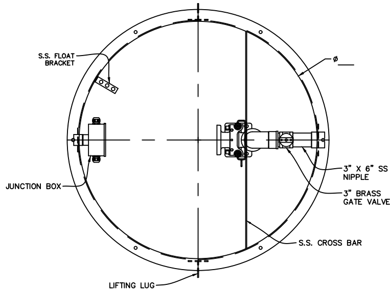
PLAN VIEW
