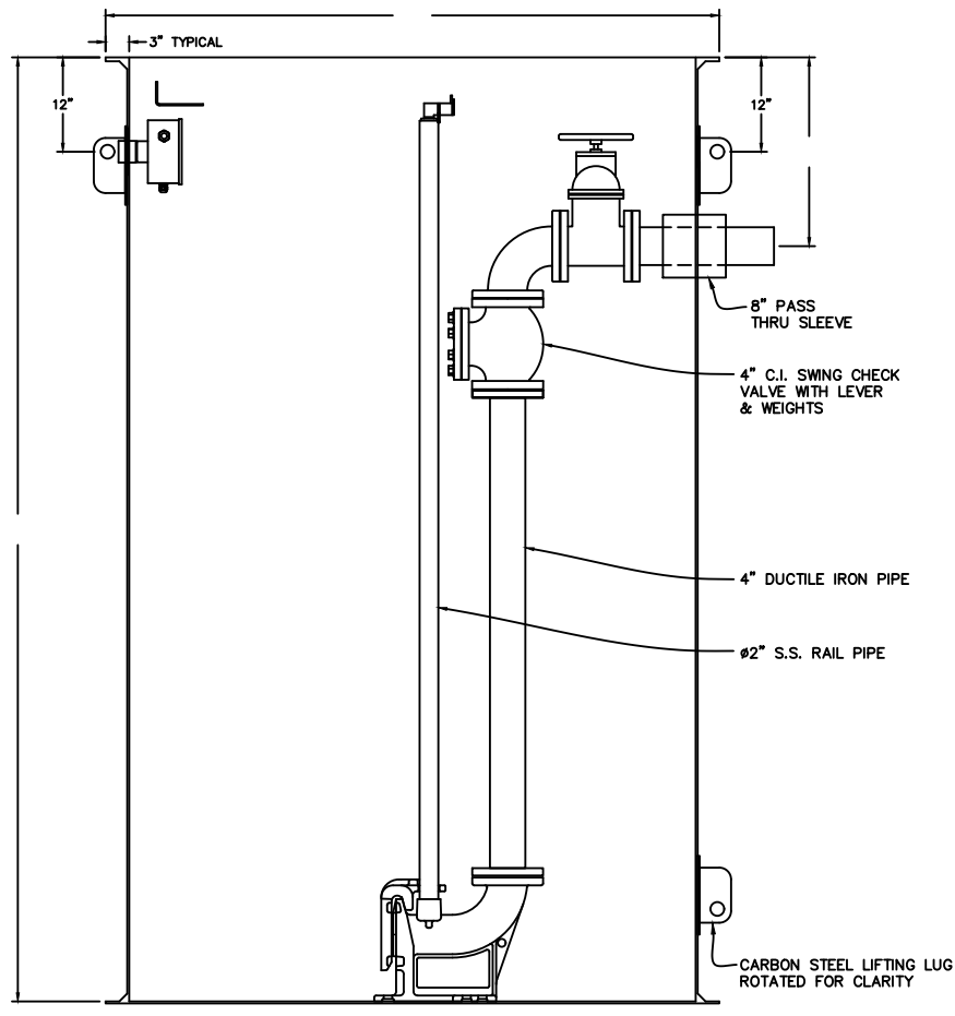
SECTIONAL ELEVATION VIEW
