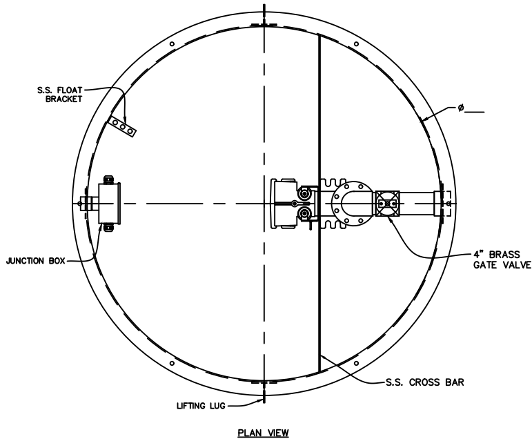
PLAN VIEW
